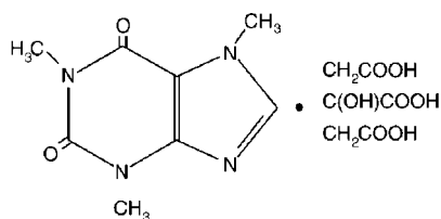
Caffeine citrate
